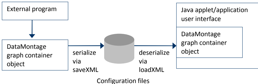
Figure 3 – Model objects simplify serialization and deserialization of DataMontage objects to/from configuration files
