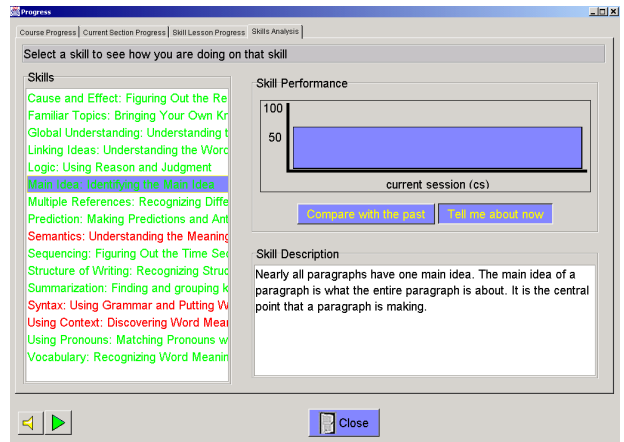
Figure 1: The tutor maintains a fine-grained assessment of the student's reading skills. It targets its remediation efforts on a learner's weak skills, here shown in red.
